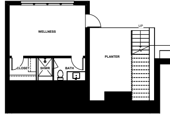
② LOWER LEVEL 3/16" = 1'-0"
