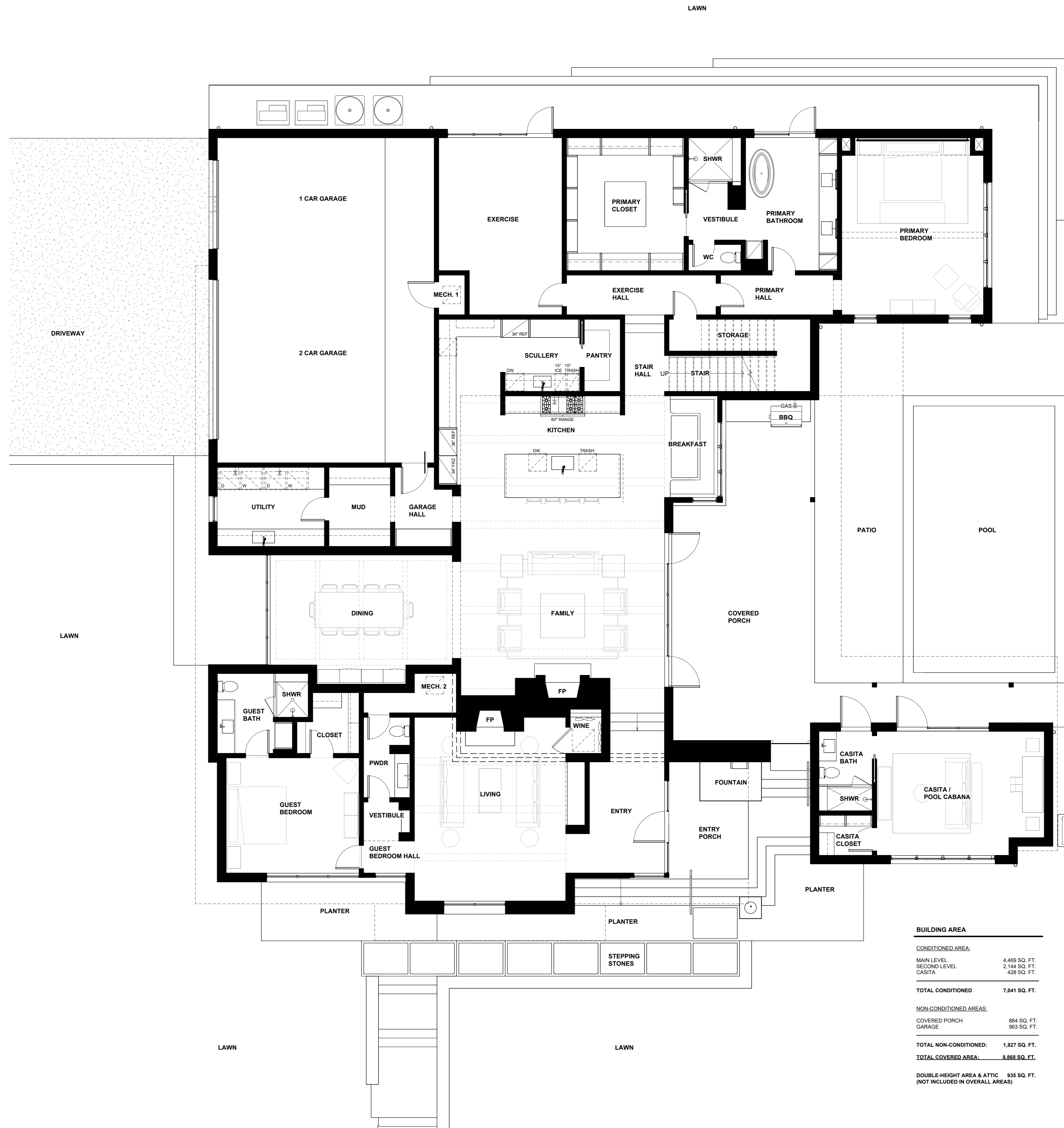
② FIRST FLOOR PLAN 3/16" = 1'-0"
